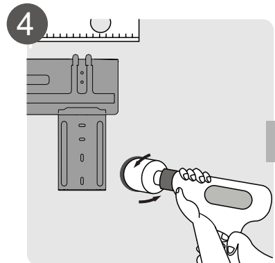
Wandloch bohren
